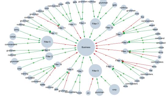
Figure 2: GAF (with attacks -; supports +) for a text classifier.
